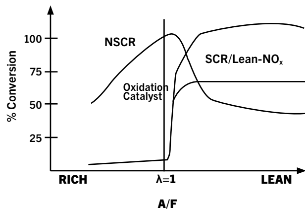
Catalyst performance for non-methane hydrocarbons (NMHCs)
