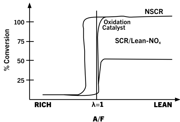
Catalyst performance for carbon monoxide (CO)
