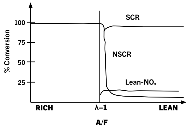
Catalyst performance for oxides of nitrogen (NO x )
